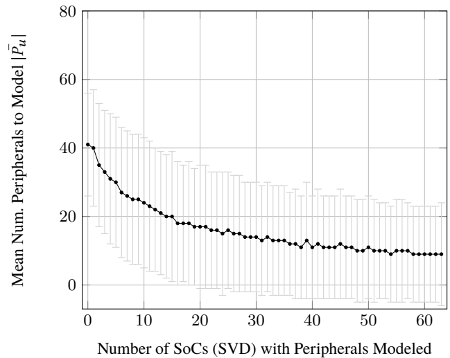
(b) Unimplemented peripherals in 64 randomly sampled Cortex systems at each round of simulation.
